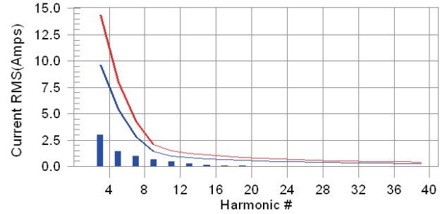
Harmonics 26: X15 230 V 50 Hz
