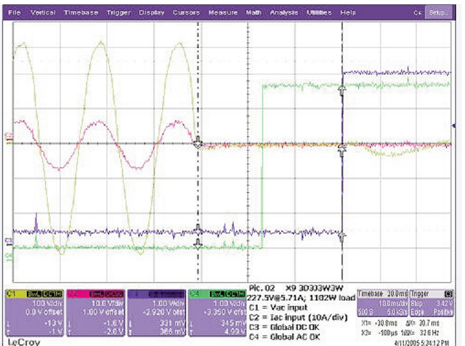
Hold Up Time X9 with 1100 W load
