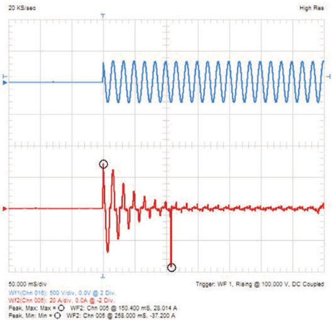
Plot 8. Inrush current for X15 at 230 VAC
