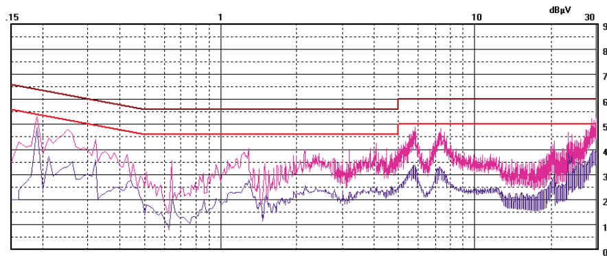
Limit #1: 55022bav Limit #2: 55022bap Detector: Peak, Average flexpower x7-3l3q2d half load v1 1i65 v2 4/4 v3 r11
