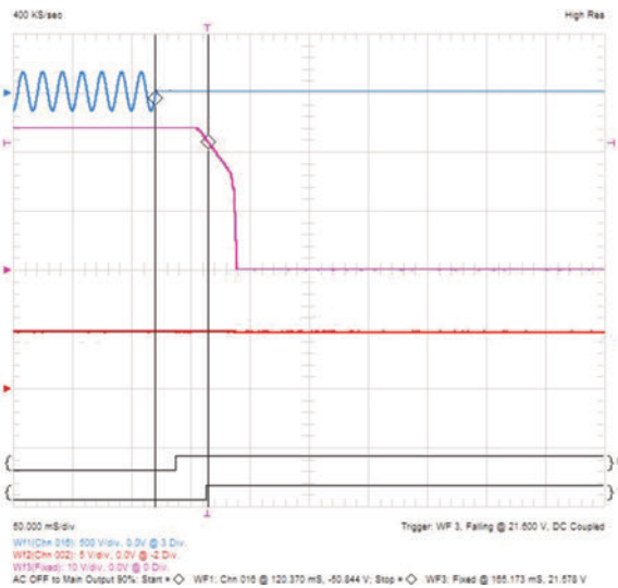
Hold Up Time X15
