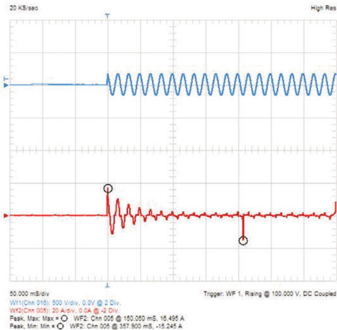
Plot 7. Inrush current for X15 at 115 VAC
