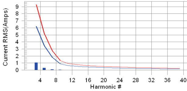
Harmonics 25: X15 120 V 50 Hz
