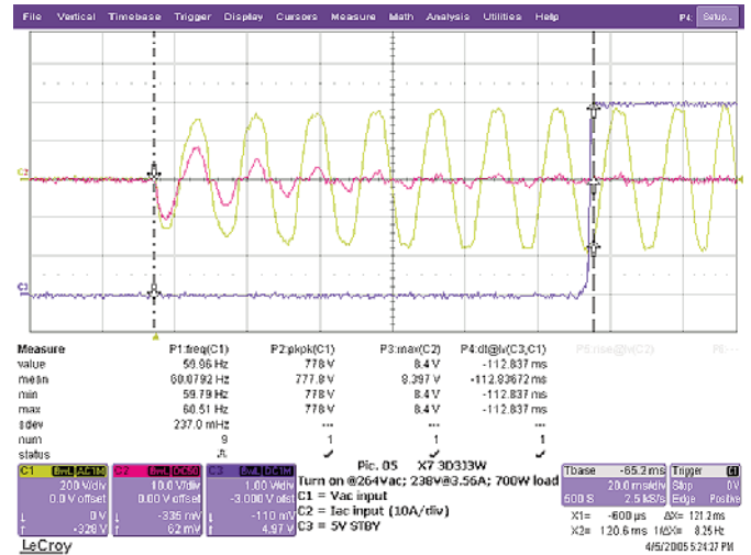
Plot 2. Inrush Current for X7 at 230 VAC
